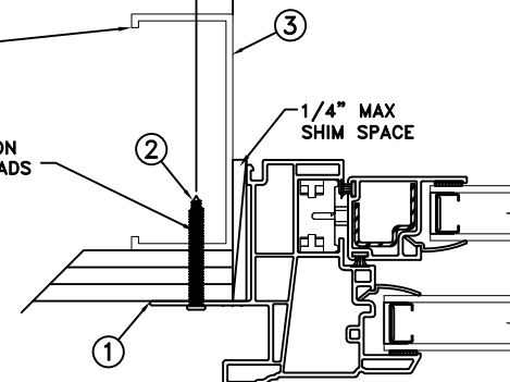
FRAME JAMB SECTION (TYP) HORIZONTAL SECTION
